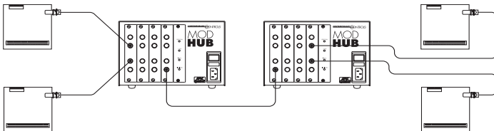
Figure 2—Active hubs can be cascaded for greater distances.
