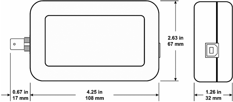
Figure 3 — USB22-CXB Dimensions
